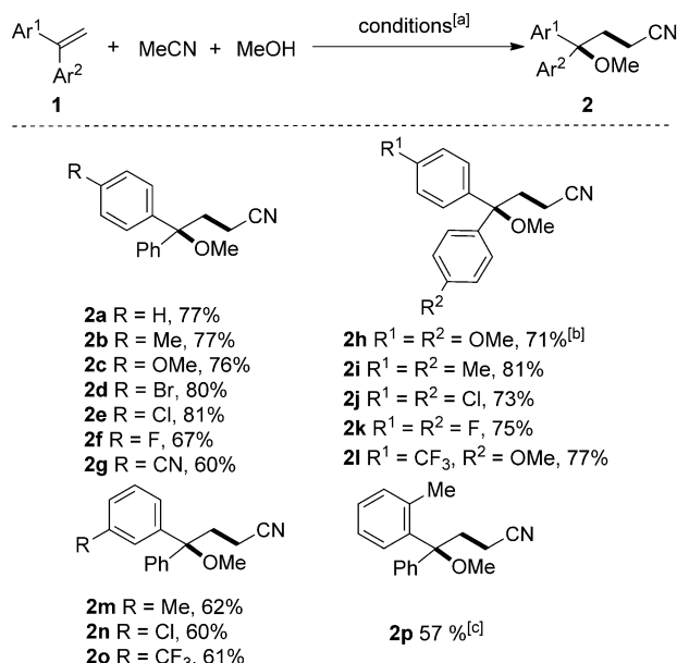
Scheme 2. Carboetherification of gem -biaryl alkenes. [a] Reaction conditions: 1 (0.50 mmol, 1 equiv), DTBP (2 equiv), Cu(OTf) 2 (0.2 equiv), 1,10-Phen (0.4 equiv), MeCN/MeOH (1:1, c 0.1 M), 120 °C, 16 h. [b] Cu(OTf) 2 (0.3 equiv) and 1,10-Phen (0.6 equiv), 24 h. [c] Cu(OTf) 2 (0.4 equiv) and 1,10-Phen (0.8 equiv) for 24 h.
