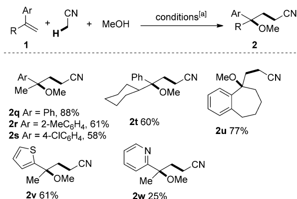
Scheme 3. Carboetherification of α-alkyl-substituted styrenes. [a] Reaction conditions: 1 (0.50 mmol), DTBP (2.0 equiv), Cu(OTf) 2 (0.2 equiv), 1,10-Phen (0.4 equiv), MeCN/MeOH (1:1, c 0.1 M), 120 °C.
